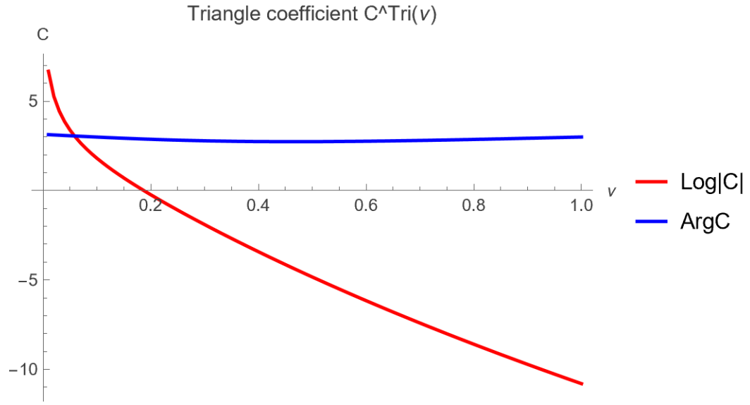
Figure 5: The coefficient C_g^{\text{Tri}}(\tilde{\nu}) defined in (33). The red and blue curves show \log |C_g^{\text{Tri}}| and \arg C_g^{\text{Tri}} in radians, respectively. The horizontal variable is \tilde{\nu} .
