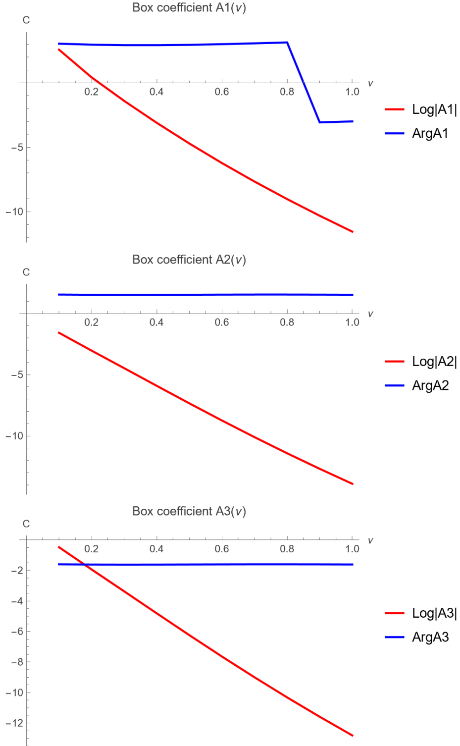
Figure 7: The angular coefficients A_{1,g} , A_{2,g} , and A_{3,g} (top to bottom) in (37) for the box diagram. Red curves show the logarithmic magnitudes and blue curves show the principal phases in radians. The horizontal variable is \tilde{\nu} .
