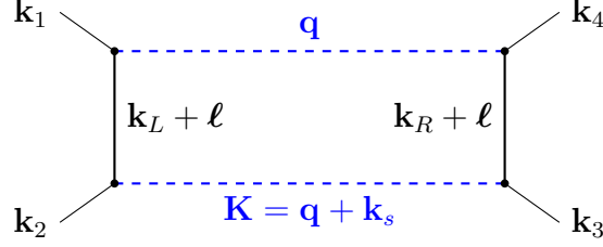
Figure 9: The double-soft region of the top-quark box. Cutting the two dashed lines separates the left and right hard exchanges. All momentum labels are vectors; the hard propagators retain their complete time dependence.
