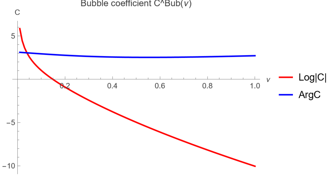
Figure 3: The bubble coefficient defined in (27). The red and blue curves show \log |C_g^{Bub}| and \arg C_g^{Bub} in radians, respectively, as functions of \tilde{\nu} .
